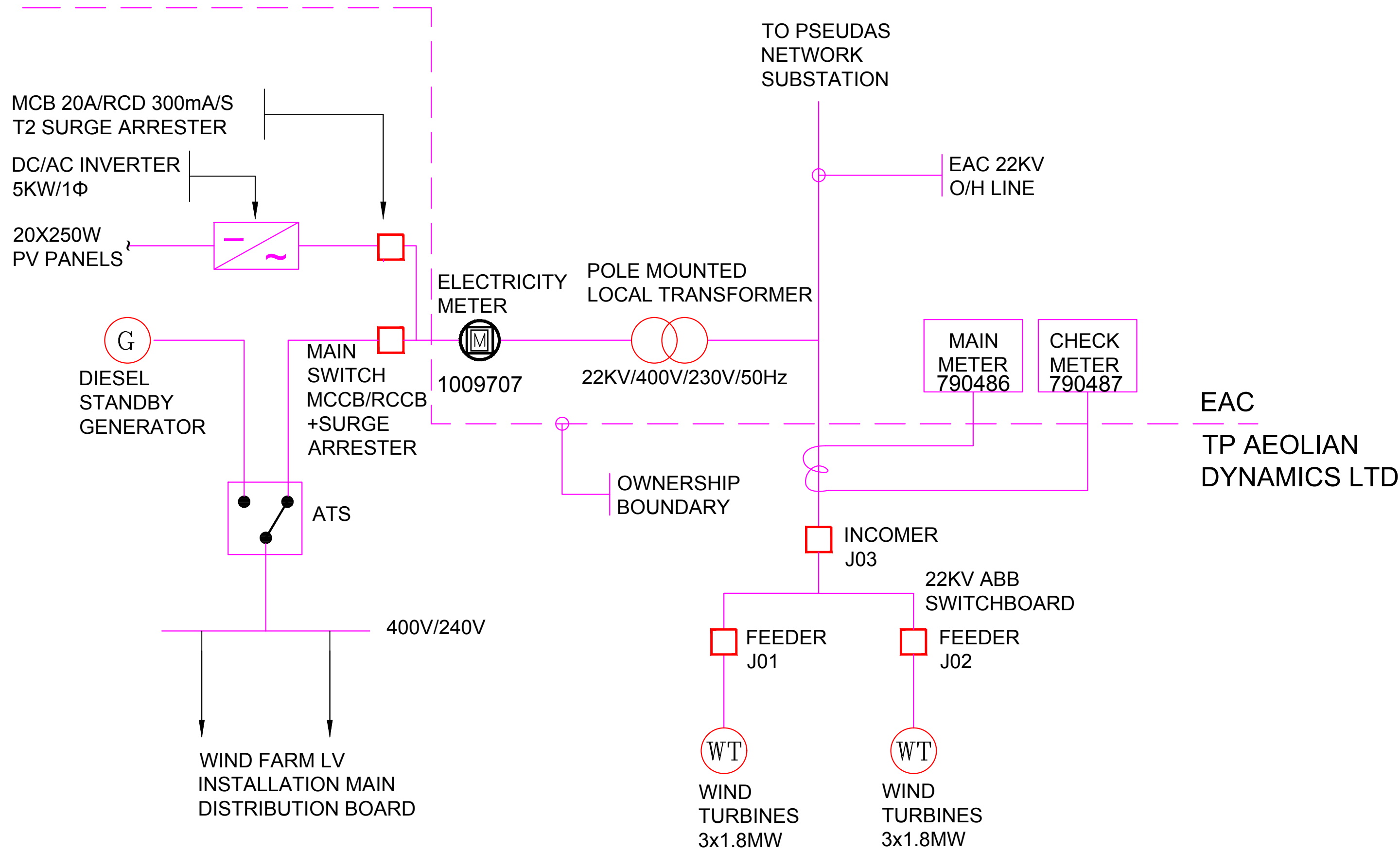
SINGLE LINE DIAGRAM
